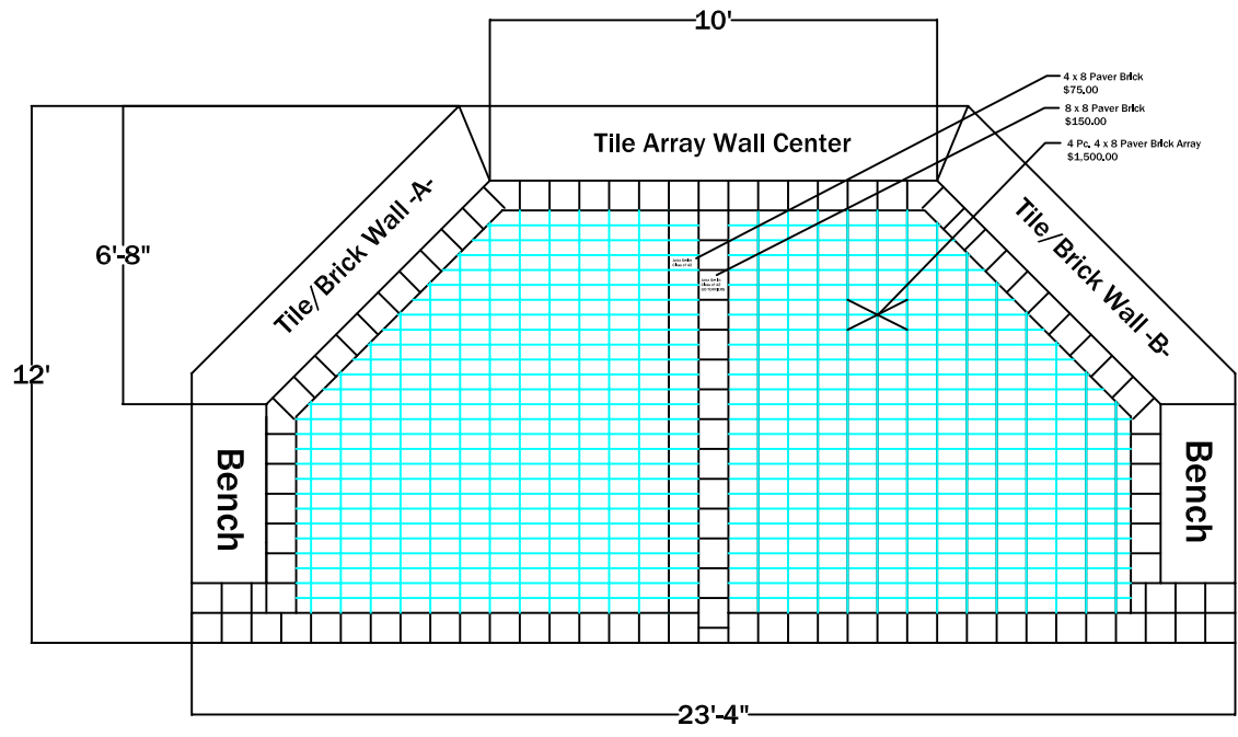
Plan View Paver Layout
